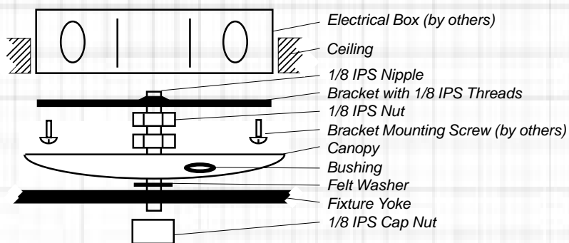
INSTALLATION DIAGRAM FOR CANOPY MOUNT FIXTURES SUPPLIED WITH SHORT NIPPLES
