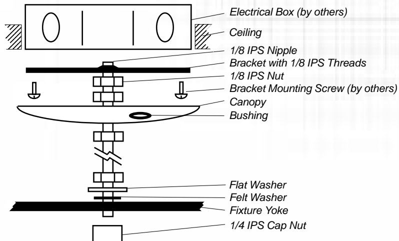
INSTALLATION DIAGRAM FOR CANOPY MOUNT FIXTURES SUPPLIED WITH LONG NIPPLES
